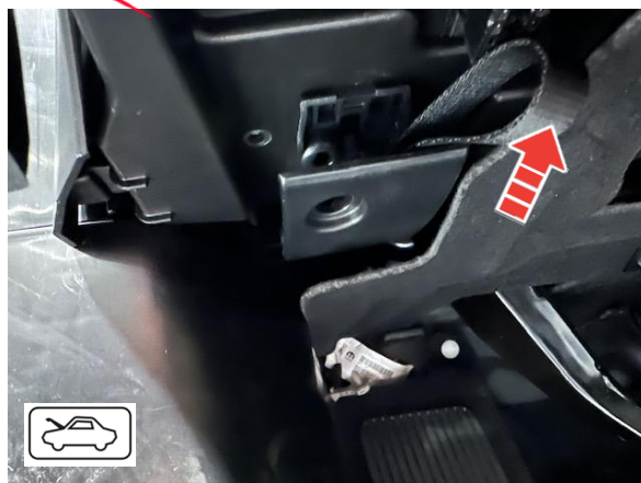
Manual Pull Strap Hood Release
